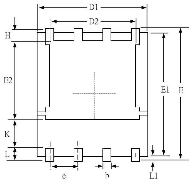
BACKSIDE VIEW
